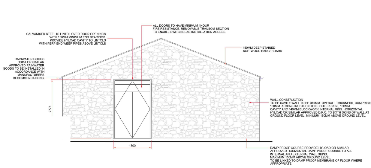
PROPOSED GABLE END (LEFT) ELEVATION
