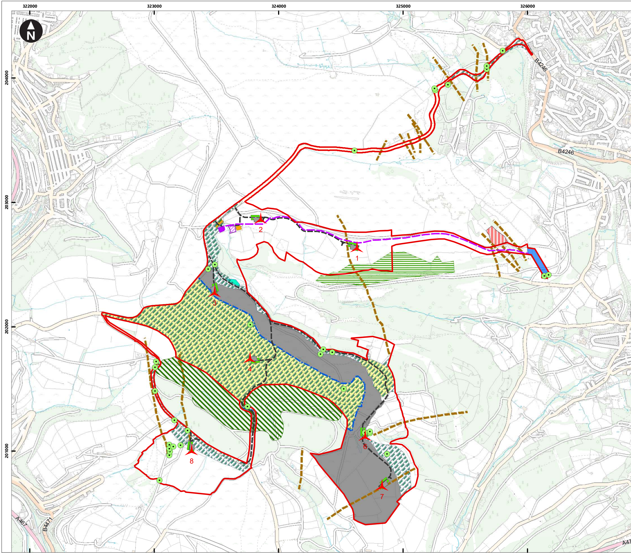
Figure 11.1 Ground conditions: ground and mining constraints
