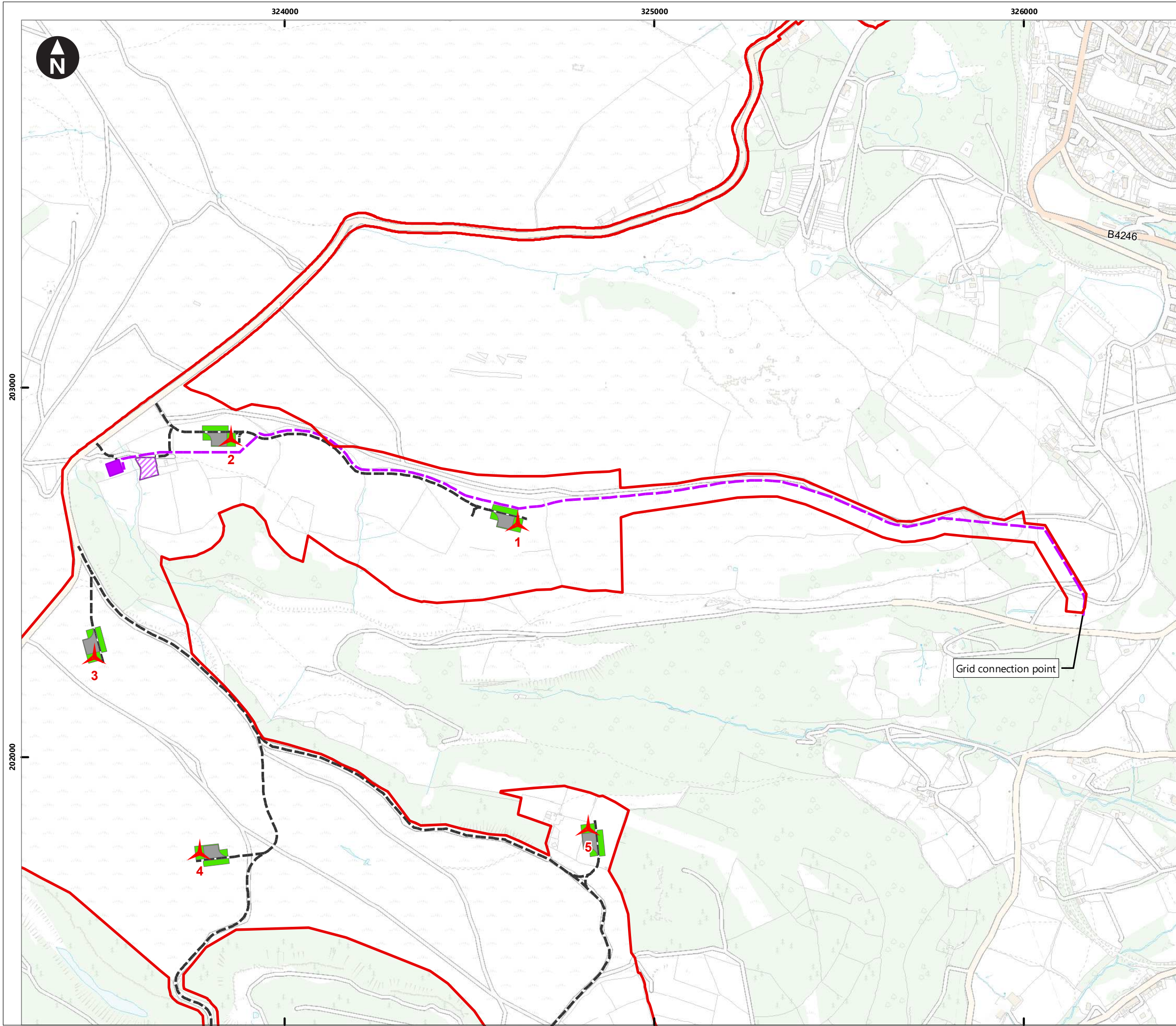
Figure 4.3 Proposed grid connection
